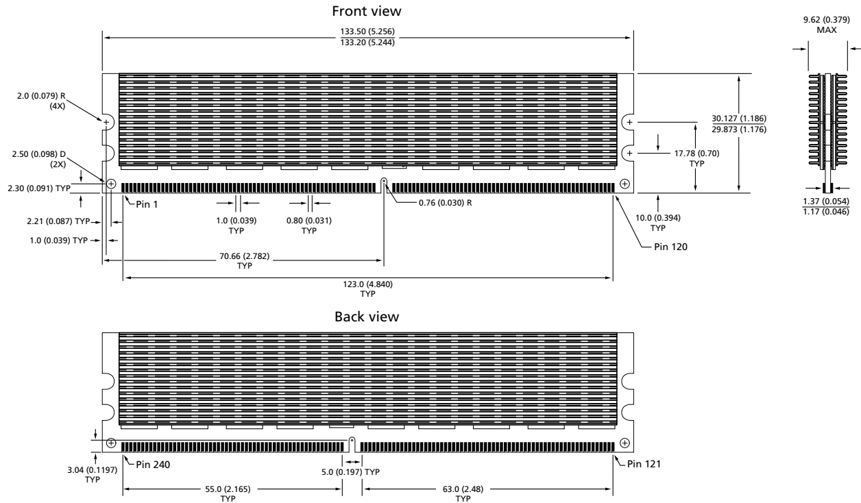
Figure 4: 240-Pin DDR2 RDIMM with Heat Spreader
