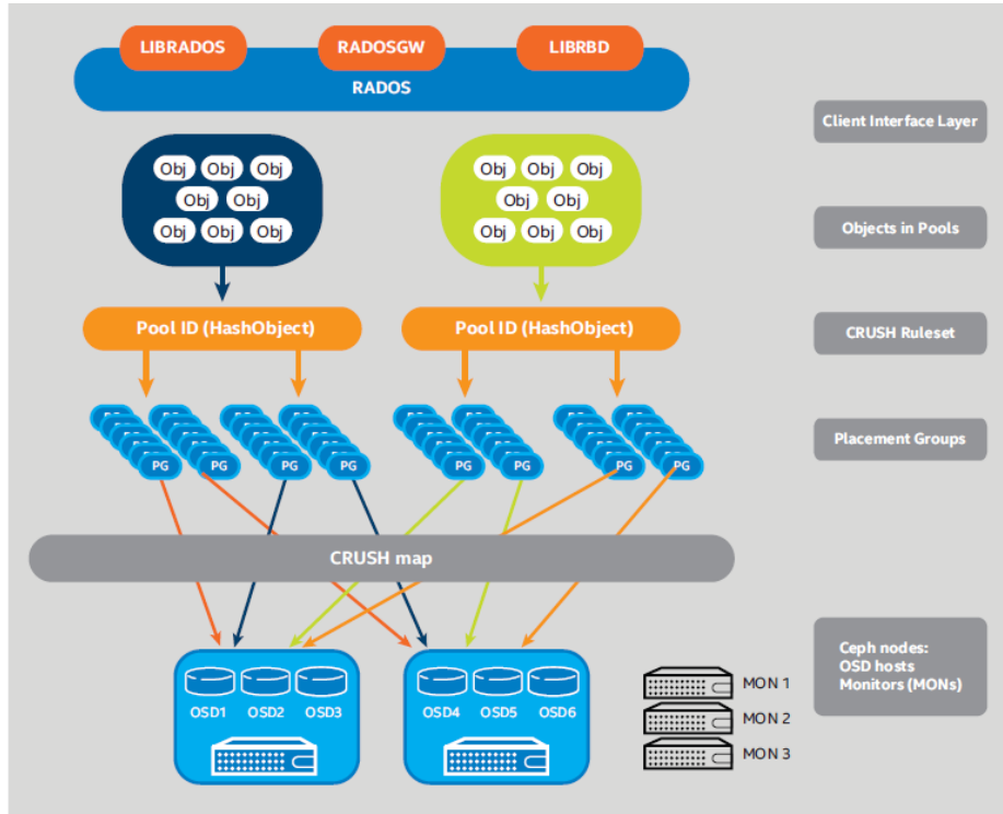
Figure 1: Ceph Architecture
