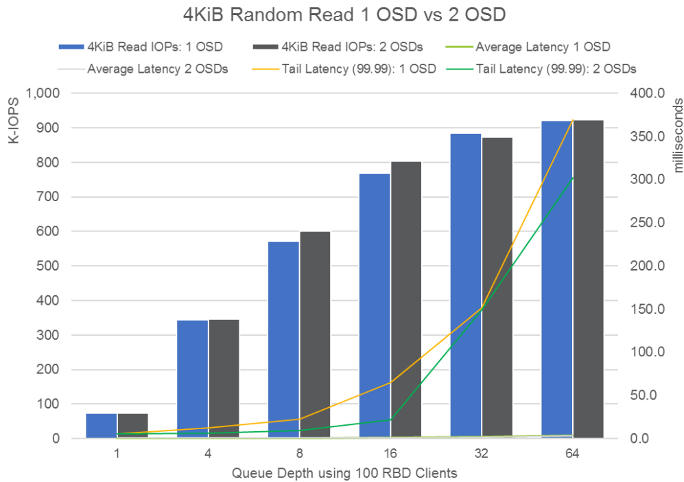
Figure 6: OSDs and Read Tail Latency
