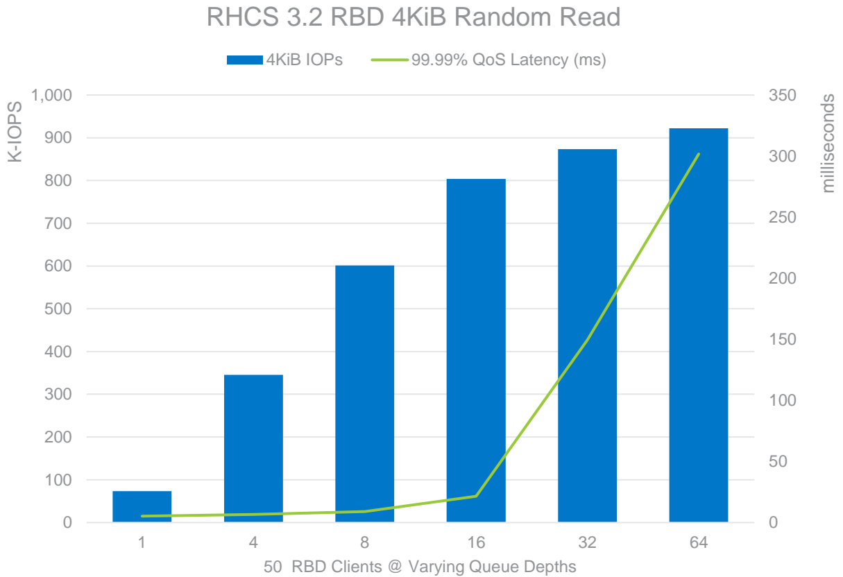
Figure 10: 4KB Random Read IOPS vs. QoS Latency
