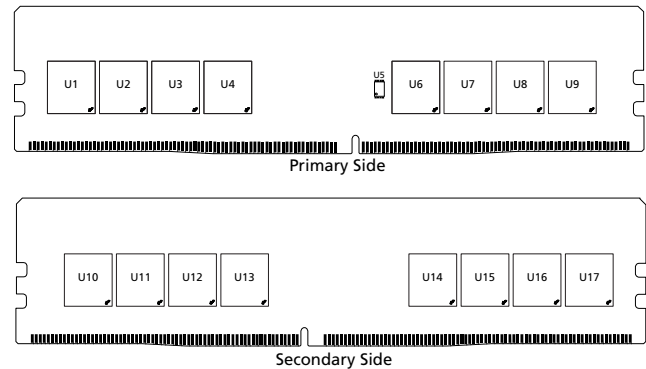
Figure 1: 288-Pin UDIMM (MO-309, R/C-B2)
